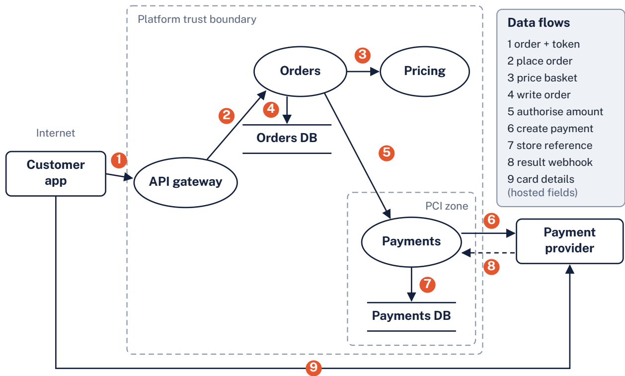
The checkout data-flow diagram with its two trust boundaries and numbered data flows.
