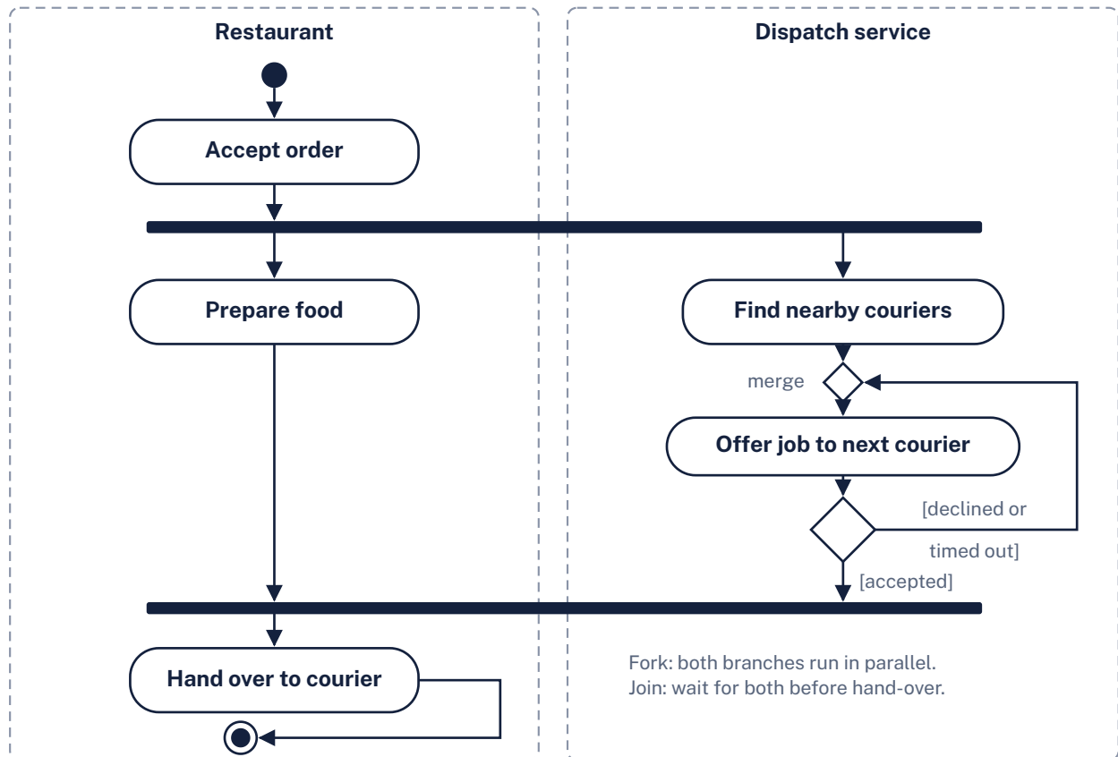
Activity diagram: from acceptance to hand-over
