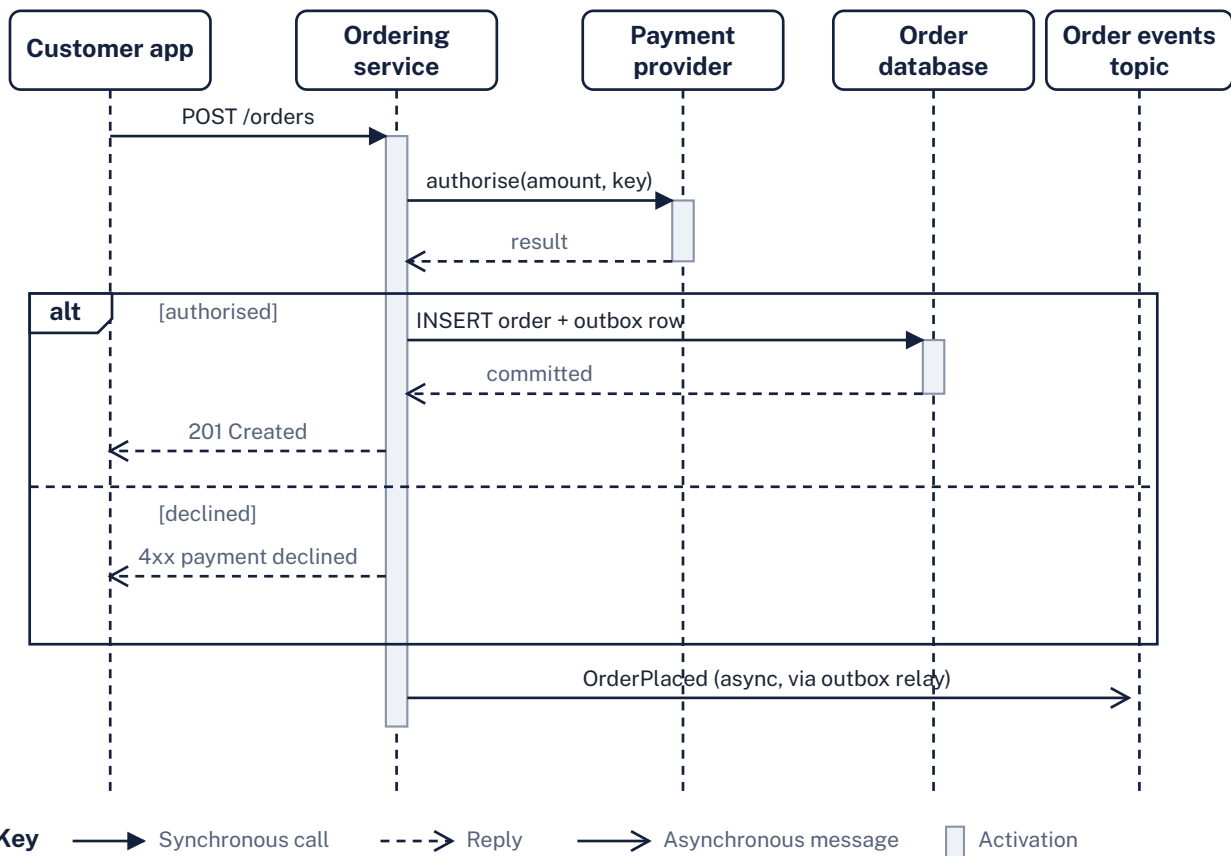
Sequence diagram: place order
