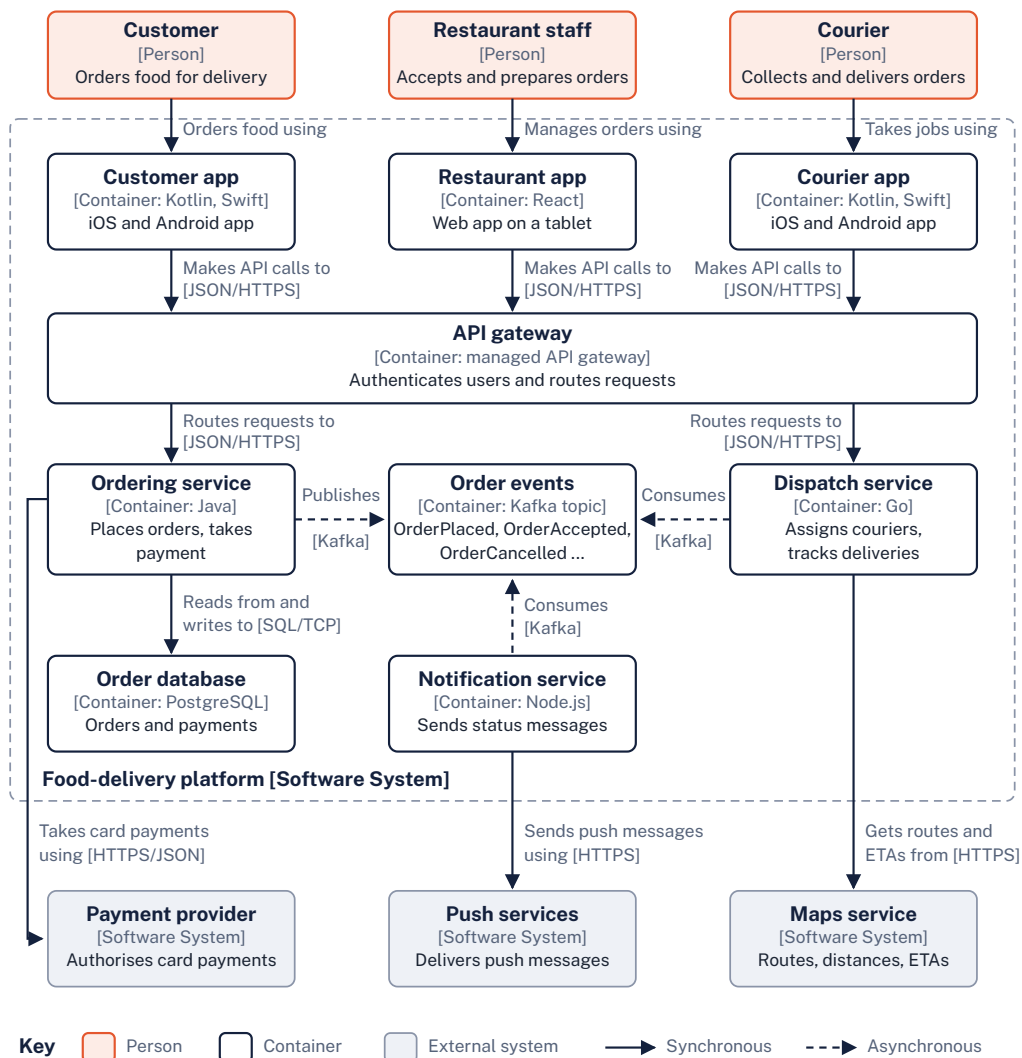
Container diagram for the food-delivery platform
