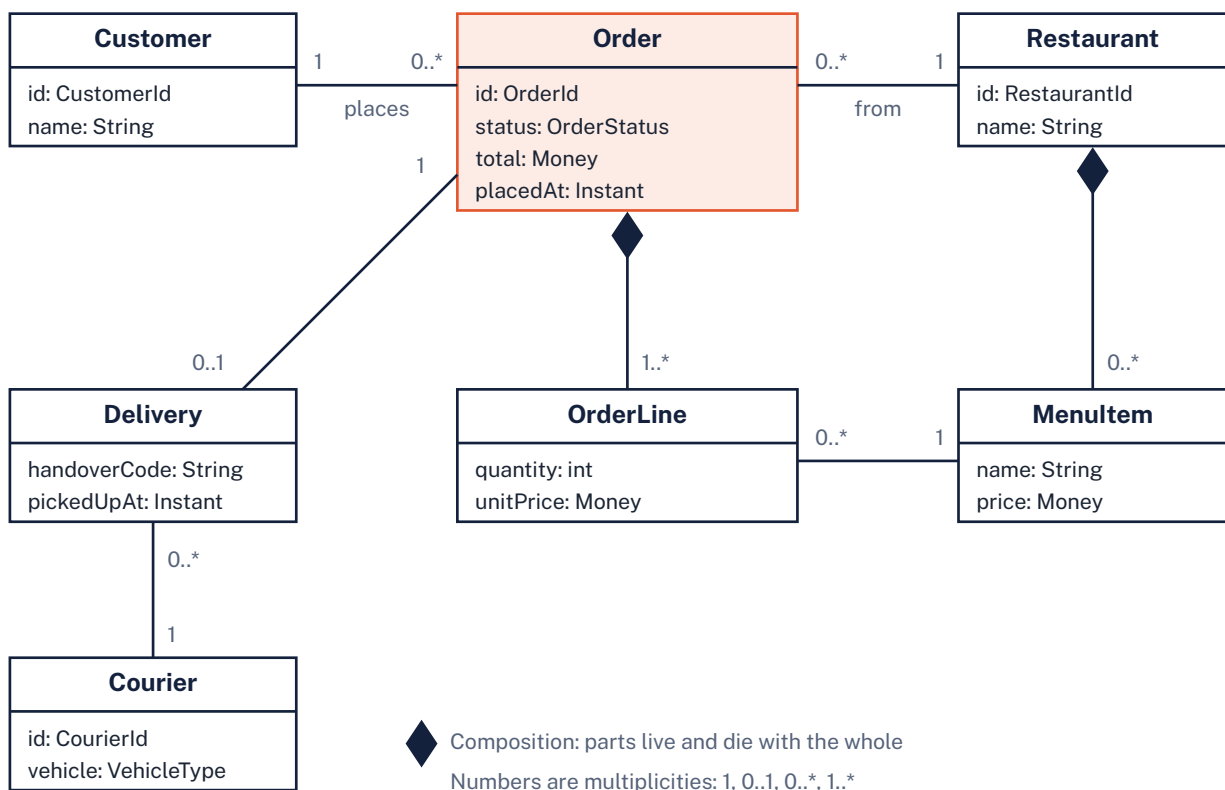
Class diagram: ordering domain model
